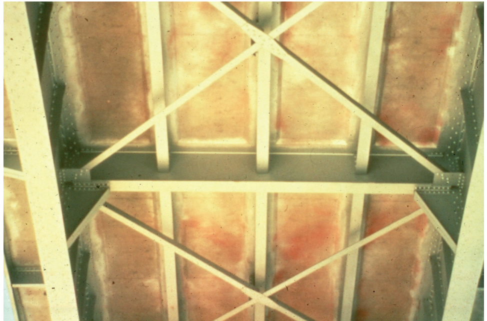
Figure P.1.39 Floor System
